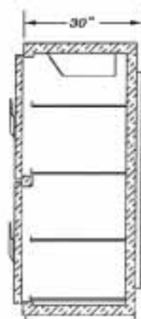
VERTICAL SECTION
