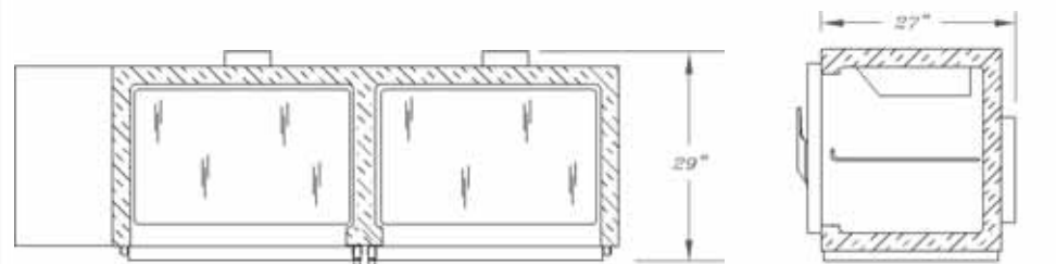
HORIZONTAL SECTION
