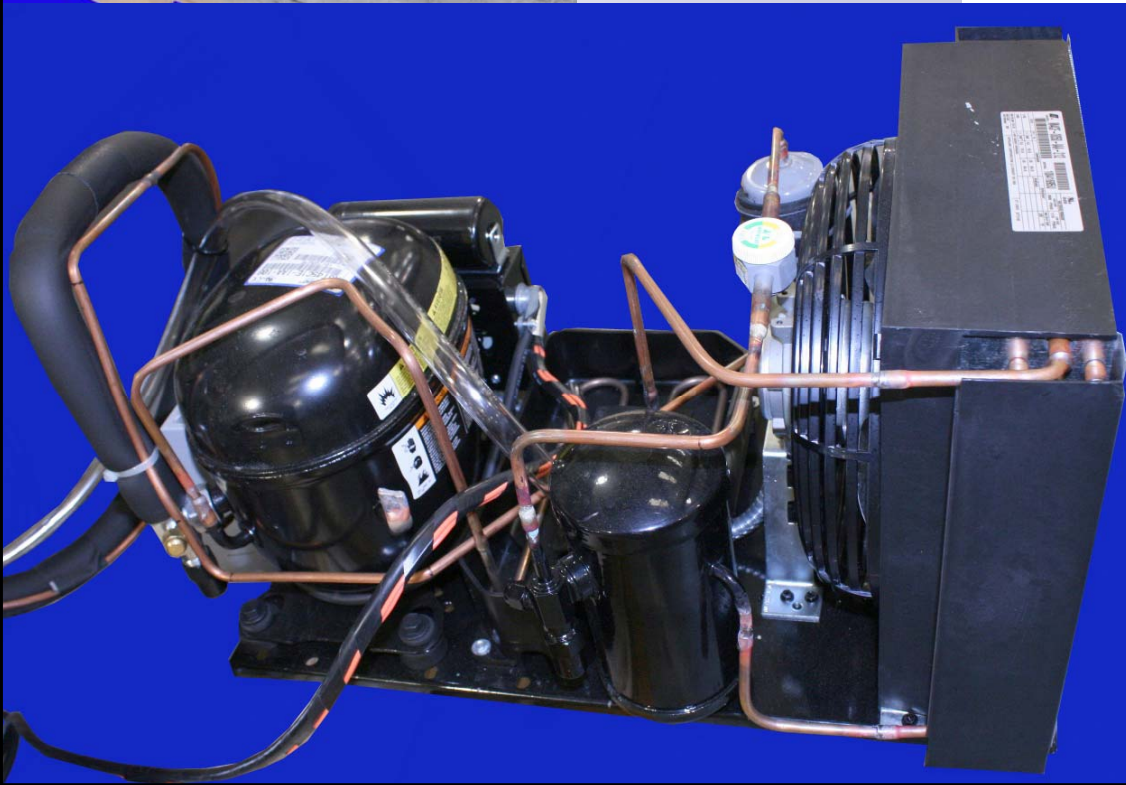
Illustration 2.B: RUT520-2-P Condensing Unit Assembly
