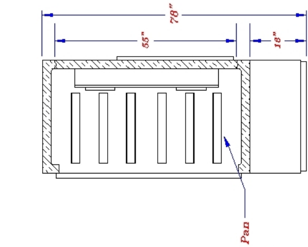
VERTICAL SECTION
