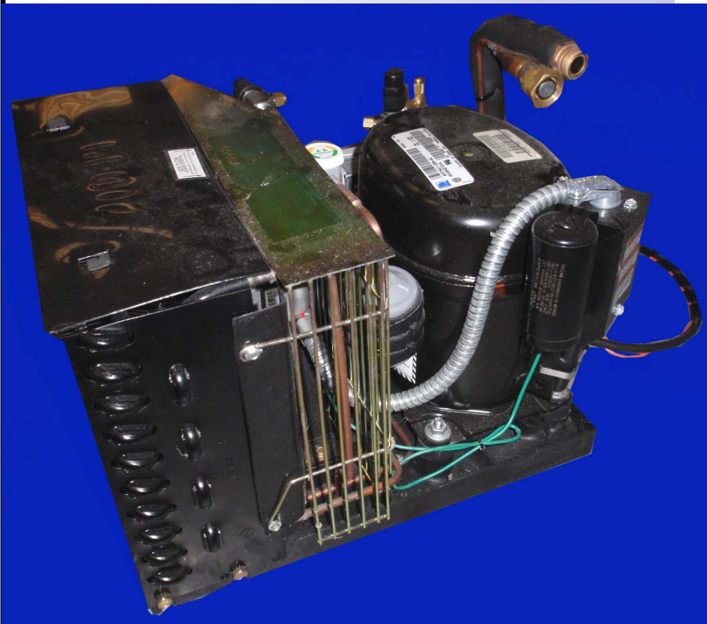
Illustration 2B RUT390-PM Condensing Unit Assembly
