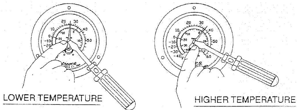
Figure 4.1 – Thermometer Calibration
